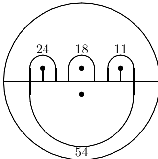
FIGURE 3. A tine edge and a noodle in D_4 .
