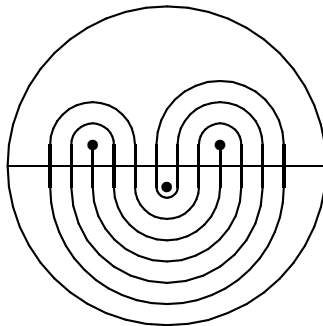
FIGURE 1. A tine edge and a noodle in D_3 .
