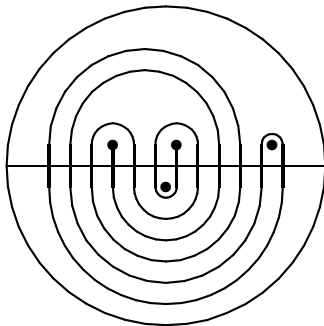
FIGURE 2. A tine edge and a noodle in D_4 .
