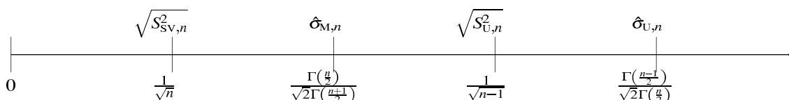
FIGURE 2. Relative positions of the estimates \sqrt{S_{SV,n}^2} , \hat{\sigma}_{M,n} , \sqrt{S_{U,n}^2} and \hat{\sigma}_{U,n} , and their coefficients.
