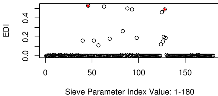
EDIs FOR IDENTIFIABILITY, n= 1000
