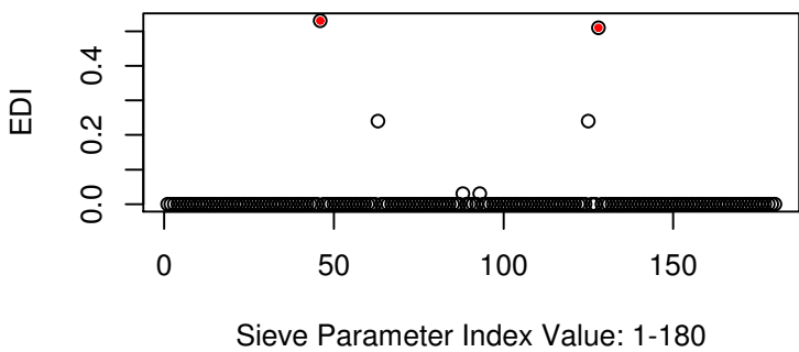
EDIs FOR IDENTIFIABILITY, n= 30000
