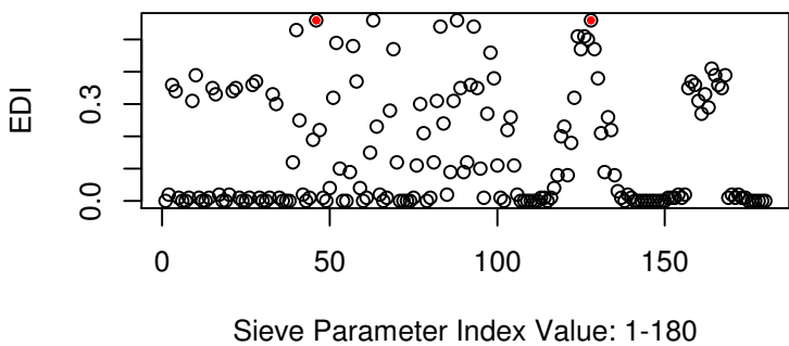
EDIs FOR IDENTIFIABILITY, n= 100
