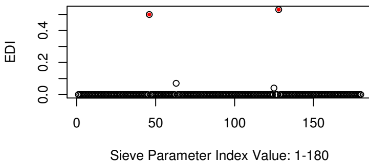
EDIs FOR IDENTIFIABILITY, n= 1e+05
